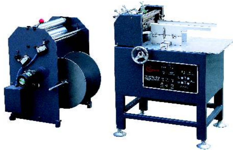
切纸机、送纸机 sheeter/paper cutter, unwinder
